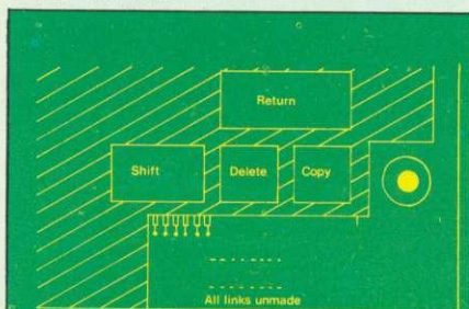
Figure 7. Keyboard links
