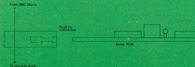
Figure 3. Side-view of drive connector
