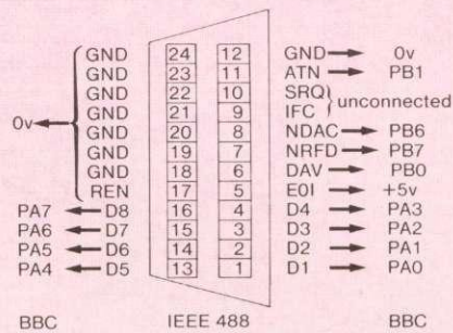
Figure 3. Interconnections between IEEE488 connector and BBC machine
